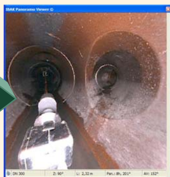
Acometida diagonal
